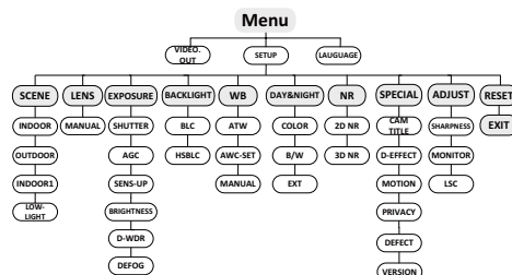
Figure 3-1 Main Menu
