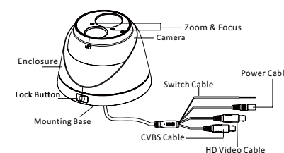
Figure 1-1 Overview of Type I Camera
