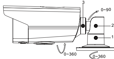
Figure 2-7 3-axis Adjustment
